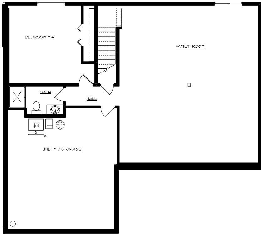
lower floor plan
